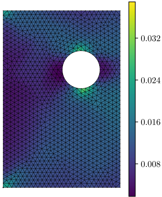
Predicted Strain \varepsilon_{xx}
