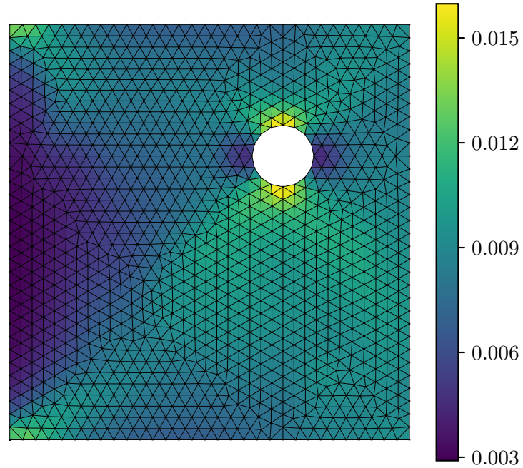
Predicted Strain \varepsilon_{xx}
