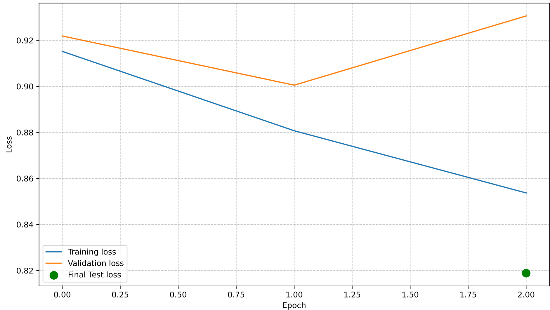
Losses Plot
