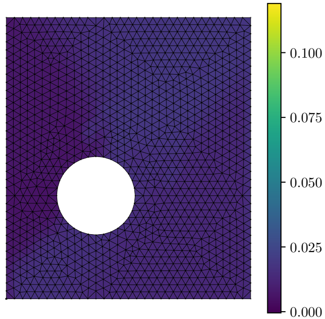
Predicted Strain \varepsilon_{xx}
