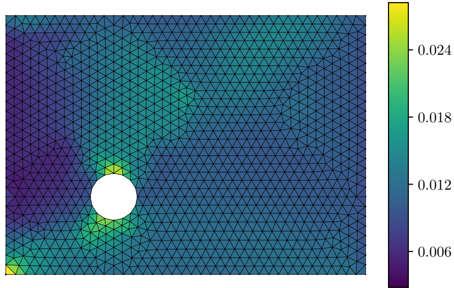
Predicted Strain \varepsilon_{xx}
