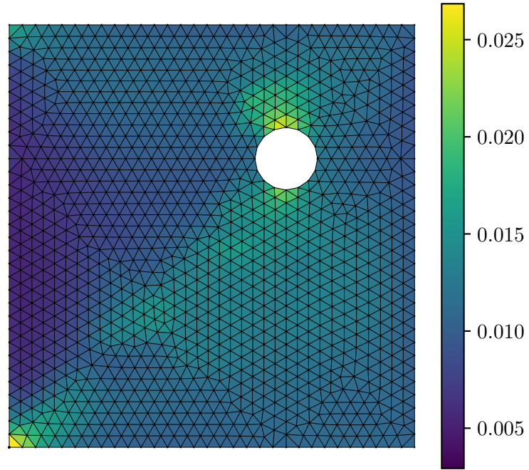
Predicted Strain \varepsilon_{xx}
