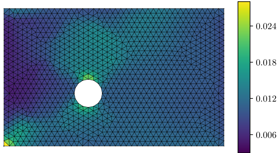
Predicted Strain \varepsilon_{xx}
