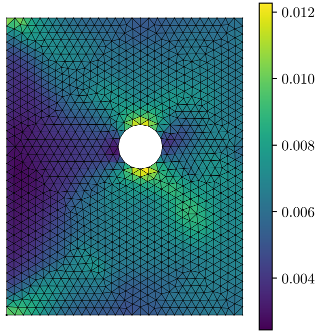
Predicted Strain \varepsilon_{xx}
