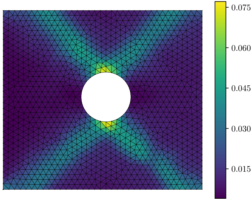
Predicted Strain \varepsilon_{xx}
