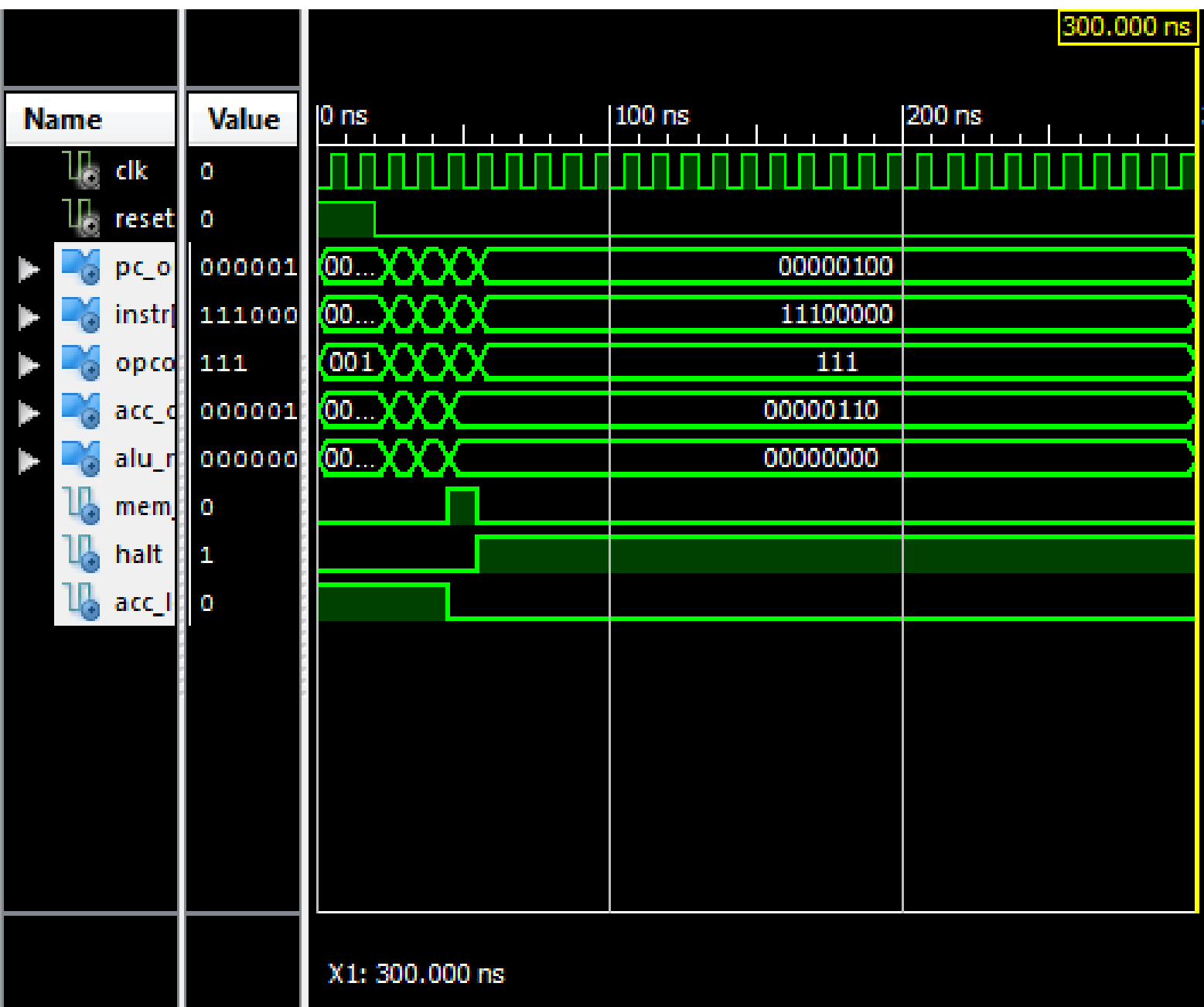
Figure 1: CPU Execution Waveform
