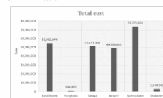
Figure 14 - Total cost for the network construction, desalination plant and O&M
