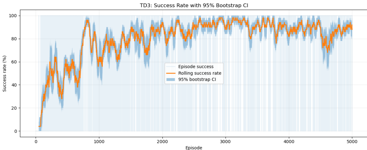
Figure 10: TD3 success over up to 100 recent training episodes. After early improvement, the rate is generally near 90%, with temporary regressions. The final 100-episode value is 89%; the final 250-episode fraction is 88.8%.
