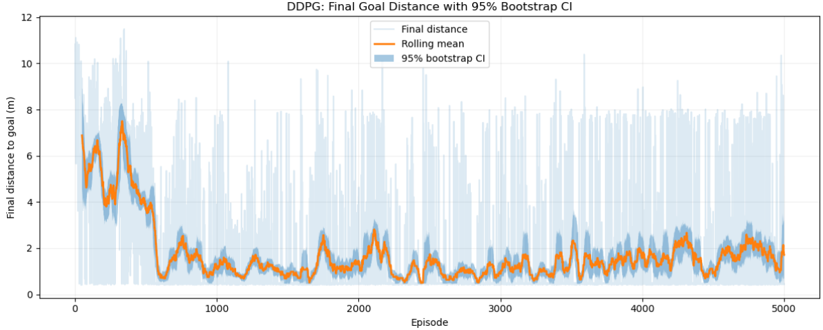
Figure 8: DDPG final goal distance in metres for all training episodes, with a rolling mean over up to 100 episodes and its 95% bootstrap confidence interval. The vertical axis spans the full range of observed distances (maximum 11.5 m).
