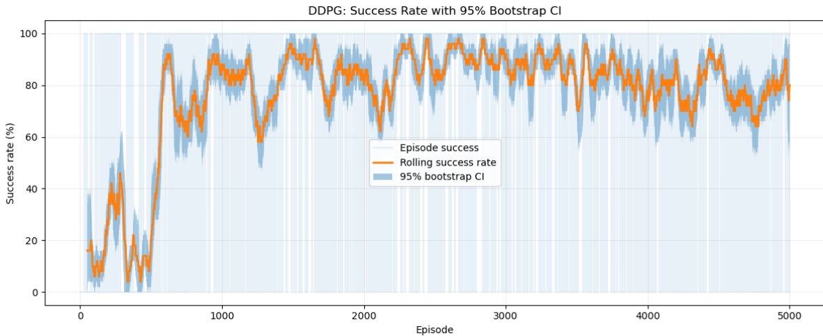
Figure 7: DDPG success rate over up to 100 recent training episodes. Success is determined by goal completion, independently of the sign of the shaped return. The final plotted value is 82%, whereas the final 250-episode success fraction is 85.2%.
