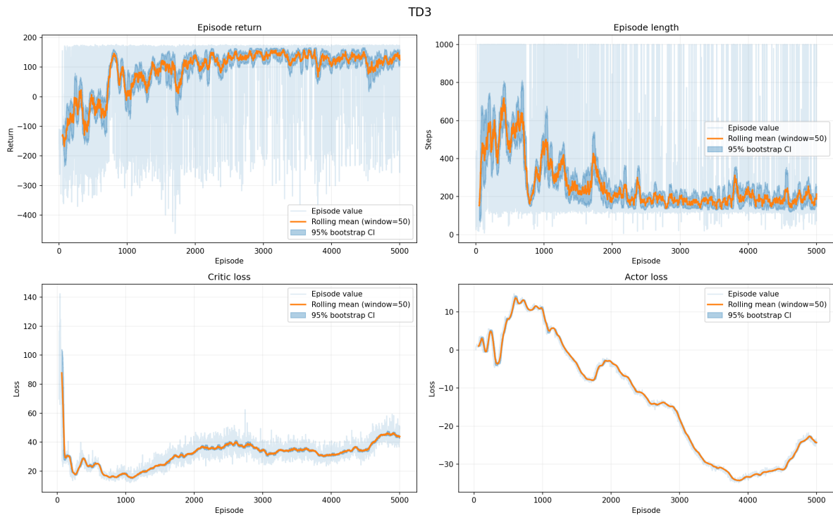
Figure 9: TD3 after tuning, over 5,000 completed episodes. Rolling return increases; episode length first rises, peaking near episode 400, then falls. Shaded bands are 95% bootstrap confidence intervals for the rolling means; actor and critic losses are optimization diagnostics.
