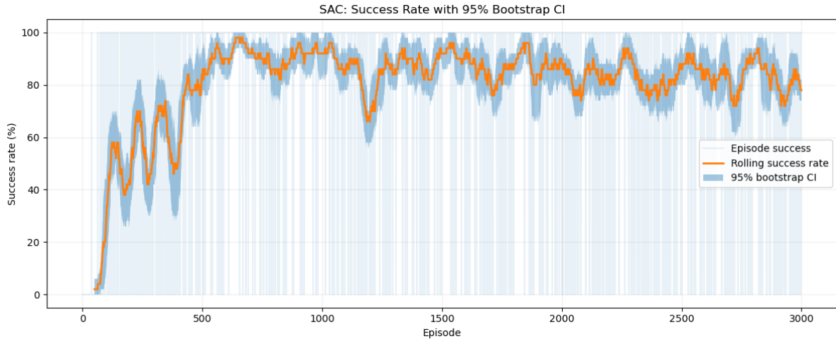
Figure 13: SAC rolling success rate with its 95% bootstrap confidence interval. The final 100-episode success rate is 79%.
