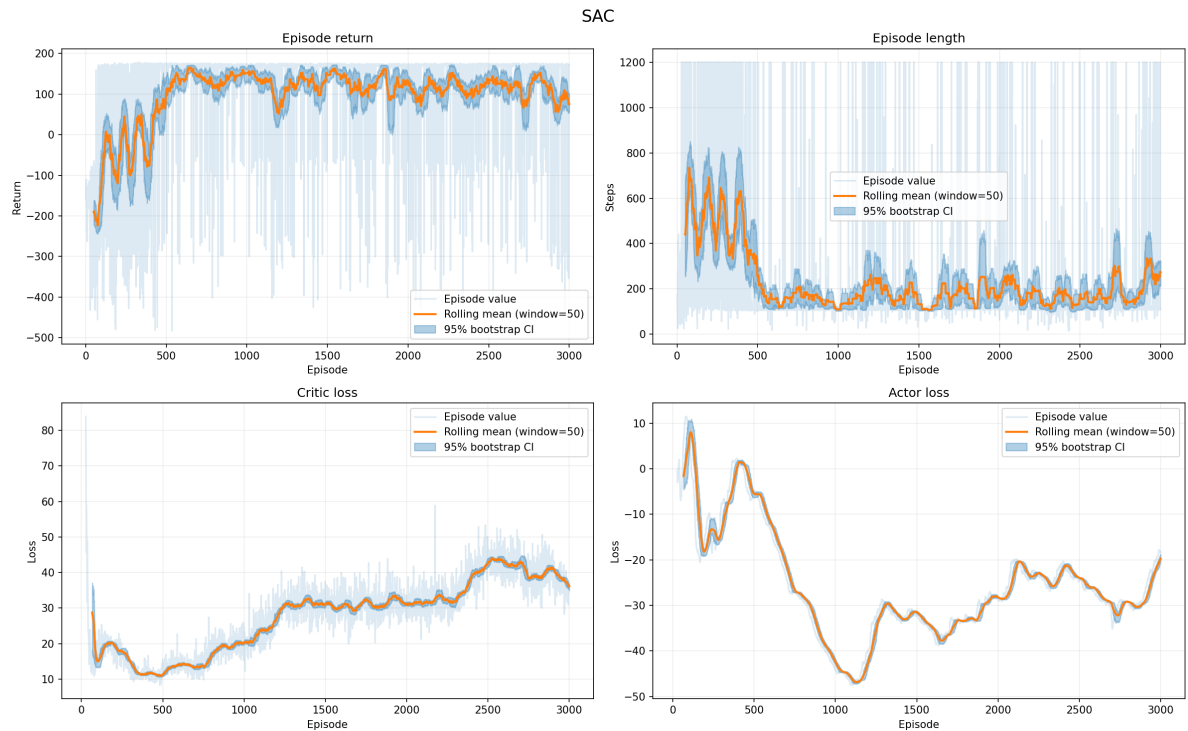
Figure 12: SAC run over 3,000 completed episodes. Return and length have rolling means with 95% bootstrap confidence intervals. The losses are episode averages and need not decrease monotonically as the policy and targets change.
