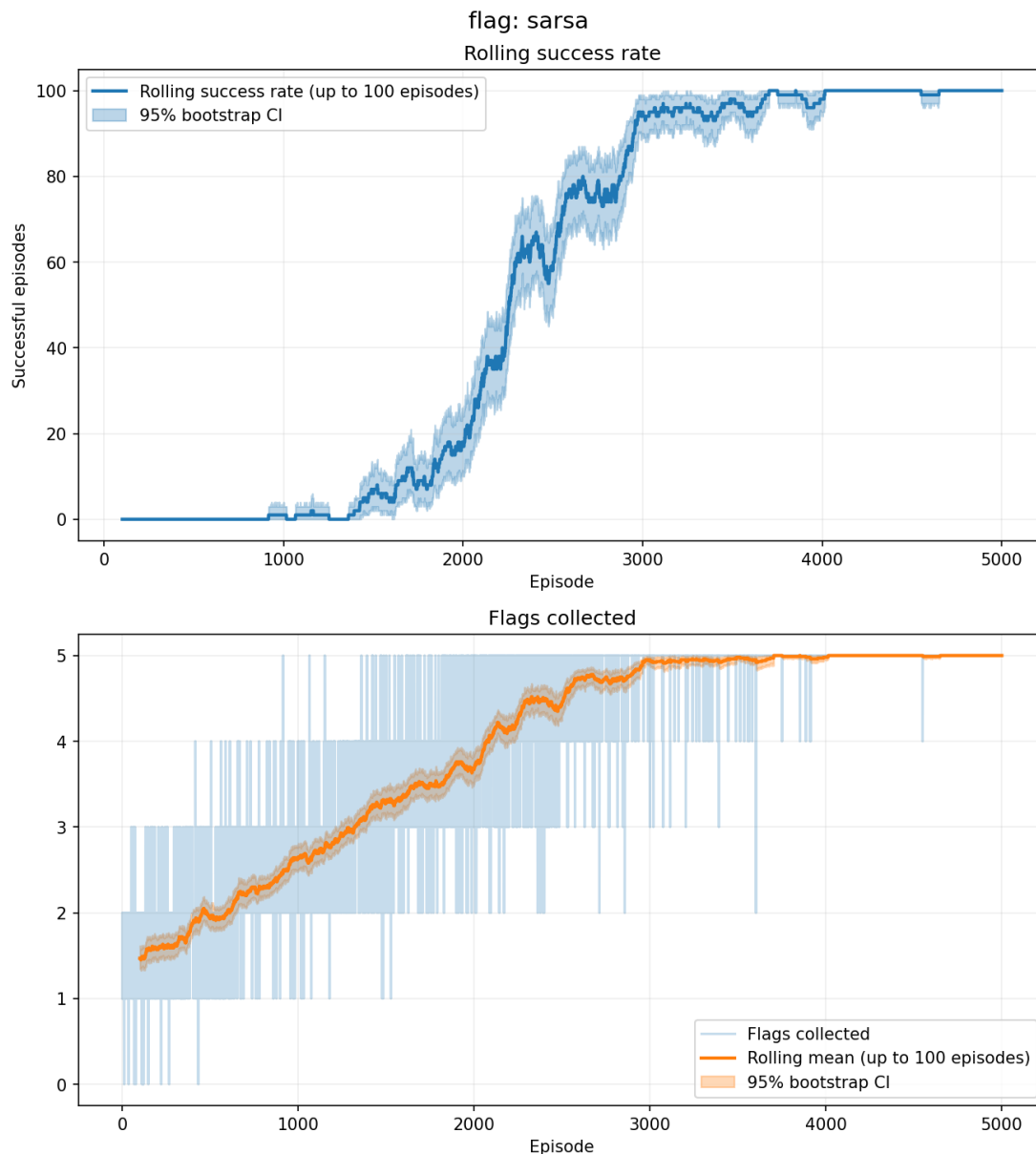
Figure 4: Flag SARSA outcomes. Occasional incomplete collections persist later in training, but all final 250 episodes collect every flag. Binary success indicators are not plotted.
