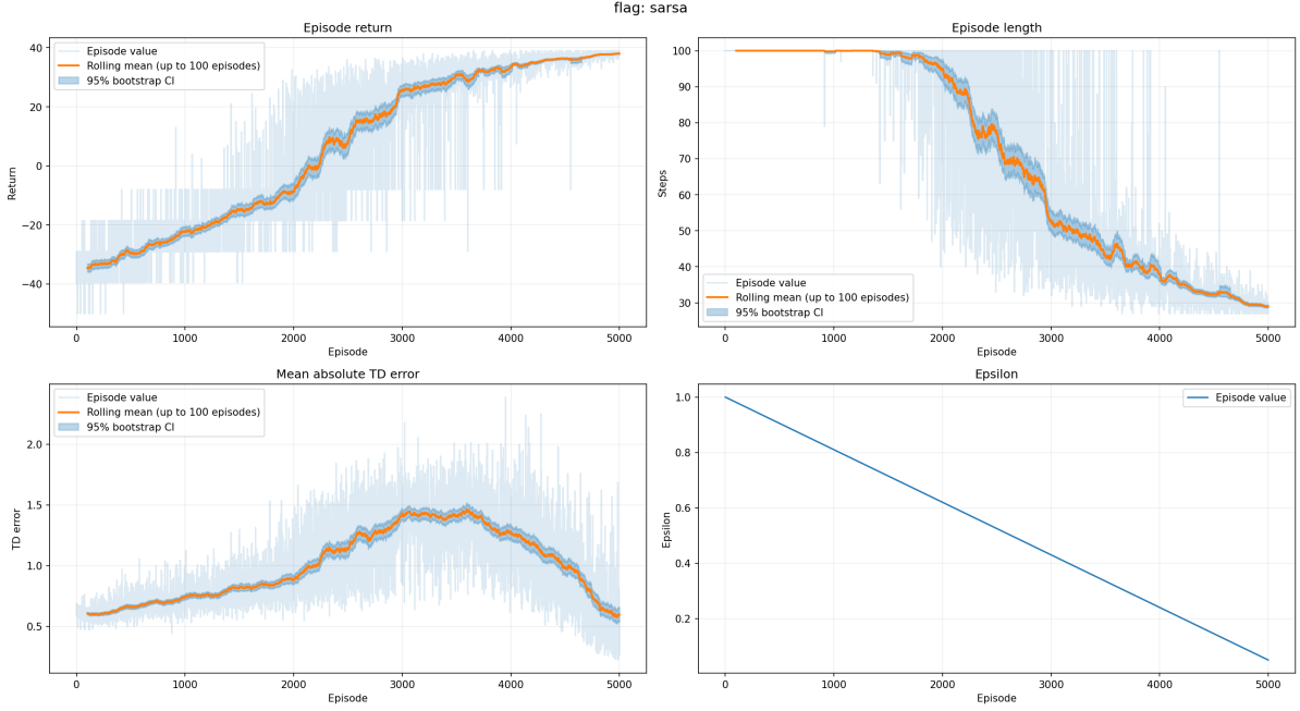
Figure 2: Flag SARSA under the same task, episode budget and exploration schedule. Successful collection becomes reliable later in this run than in the Q-learning run; sampled TD errors remain variable even after returns improve.
