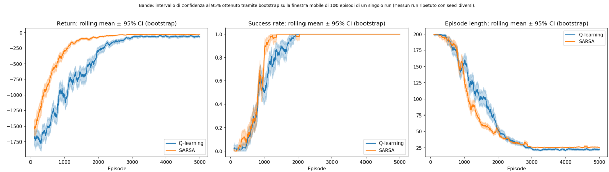
Figure 5: Cliff training comparison from the two completed 5,000-episode, seed-0 runs. SARSA achieves less negative training returns. Both eventually reach the goal reliably, while Q-learning has shorter late-training episodes but pays more cliff-fall penalties. The curves are rolling means with 95% bootstrap confidence intervals computed within each run; they show no variation across training seeds.
