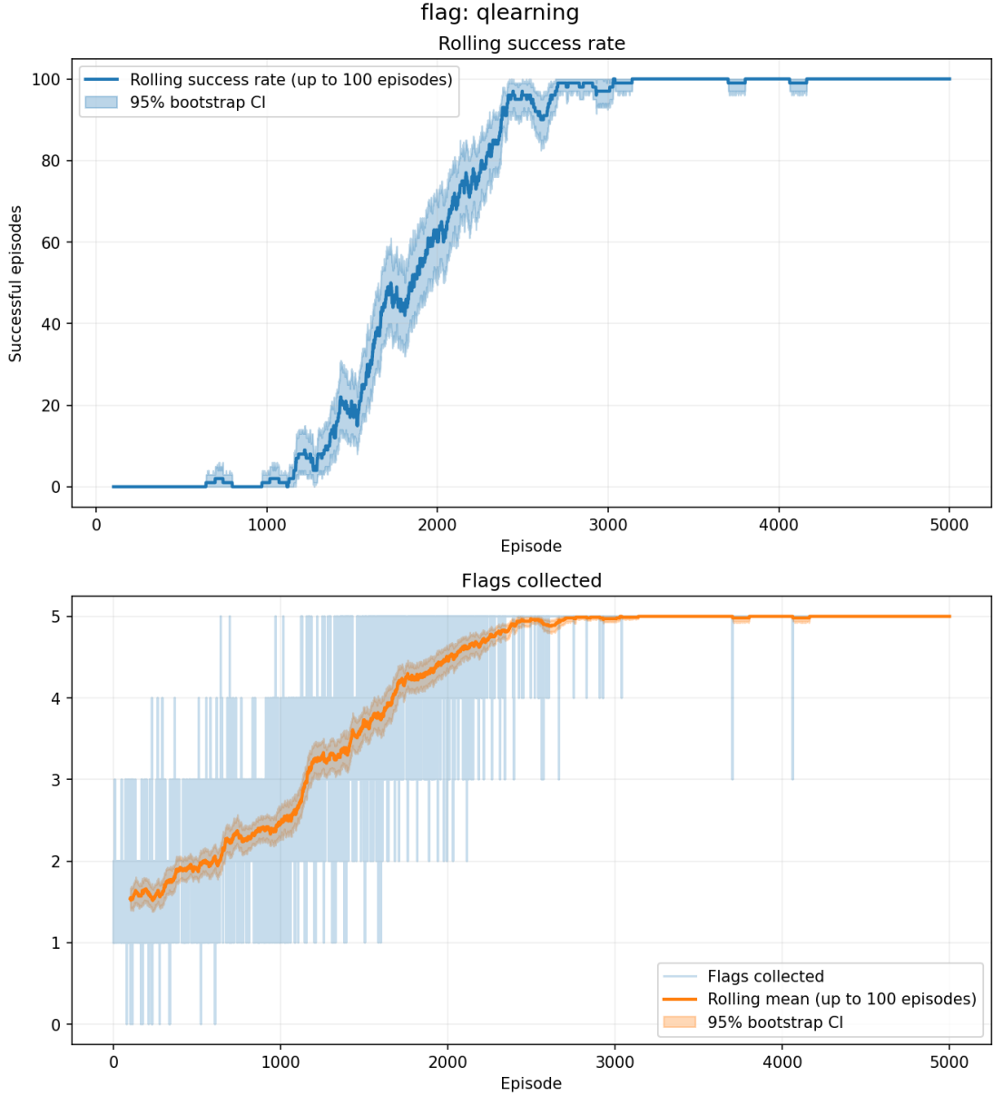
Figure 3: Flag Q-learning outcomes. The upper panel averages full-task completion over up to 100 episodes; the lower panel counts flags collected in each episode. Both distinguish partial collection from completing all five flags.
