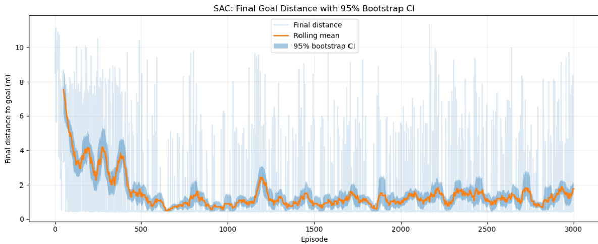
Figure 14: SAC final distance for all training episodes, with a rolling mean over up to 100 episodes and a horizontal span of 3,000 episodes. The vertical axis spans the full range of observed distances (maximum 11.3 m).
