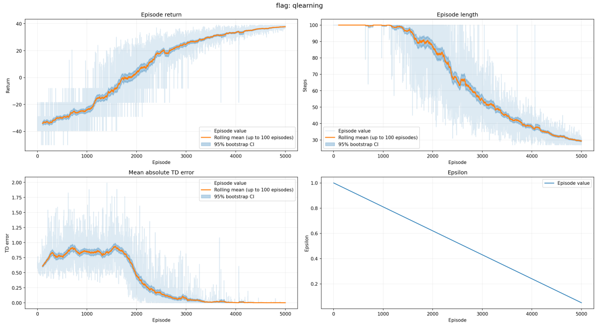
Figure 1: Flag Q-learning, 5,000 episodes with seed 0. Return and length improve as training proceeds and exploration declines. The shaded band is a 95% bootstrap confidence interval for the rolling mean.
