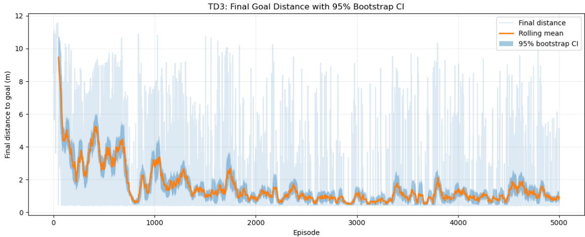
Figure 11: TD3 final goal distance. The rolling mean falls toward approximately 1 m, while occasional failures end farther from the goal. The vertical axis spans the full range of observed distances (maximum 11.6 m).
