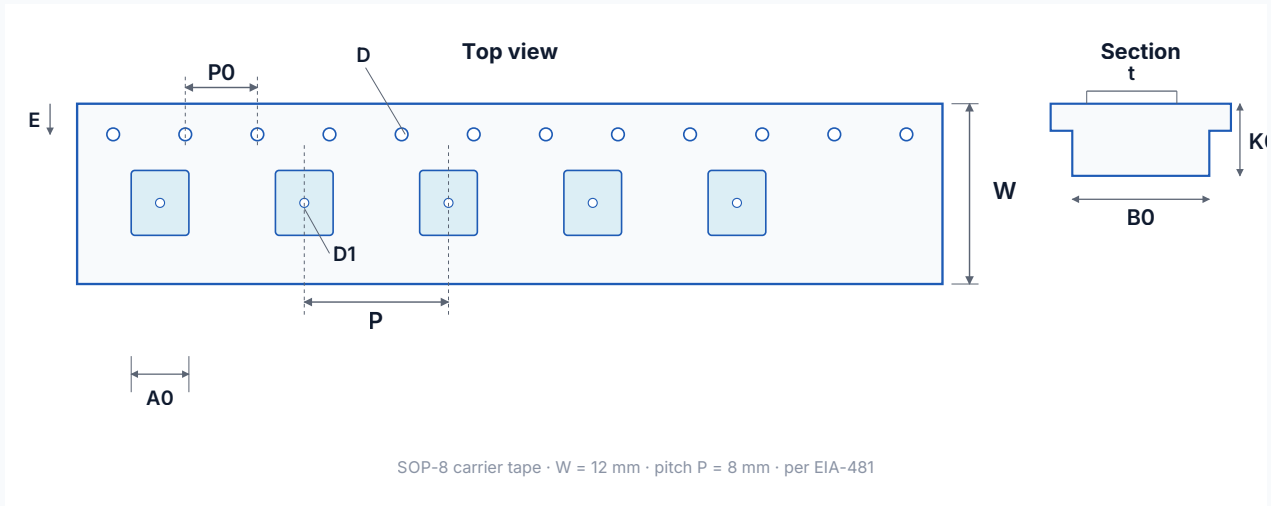
Figure 16: 12 mm carrier tape
