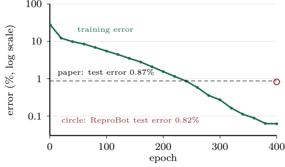
(a) MLP with L2-SVM loss, MNIST
