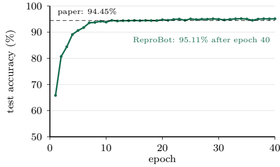
(e) Soft decision tree, MNIST
