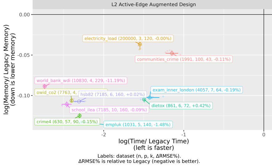
Figure 7: Runtime-memory Pareto plot for the L2 active-edge augmented-design builder. Each point compares active-edge construction with the full-pairwise L2 reference on the same dataset. Left is faster, down is lower peak memory, and labels report dataset, number of groups, and percent RMSE change.
