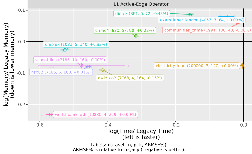
Figure 6: Runtime-memory Pareto plot for the exact L1 active-edge operator. Each point compares the operator solver with the full-edge L1 reference on the same dataset. Left is faster, down is lower peak memory, and the lower-left quadrant indicates improvement on both efficiency axes.
