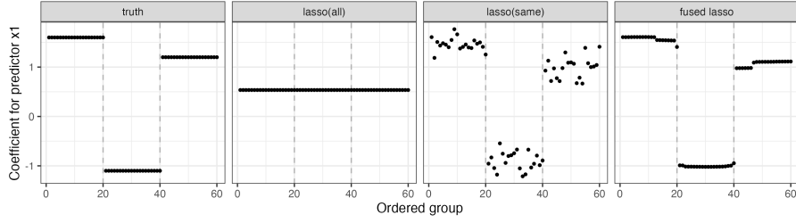
Figure 4: Controlled changepoint example comparing fused regression with unfused lasso baselines. Points show the coefficient for the first predictor across all 60 ordered groups, and dashed vertical lines mark the true changepoints. lasso(all) fits only one shared coefficient path, lasso(same) produces noisy separate paths, and the fused lasso model recovers the piecewise-constant coefficient structure. The lasso baselines are fit with glmnet .
