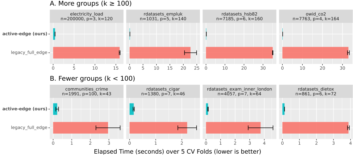
Figure 7: L2 fit time by solver and group-count regime. The active-edge builder reduces augmented-design construction when the graph is sparse.
