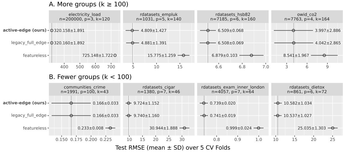
Figure 6: L2 prediction accuracy relative to the legacy L2 augmented-design solver across the benchmark panel.
