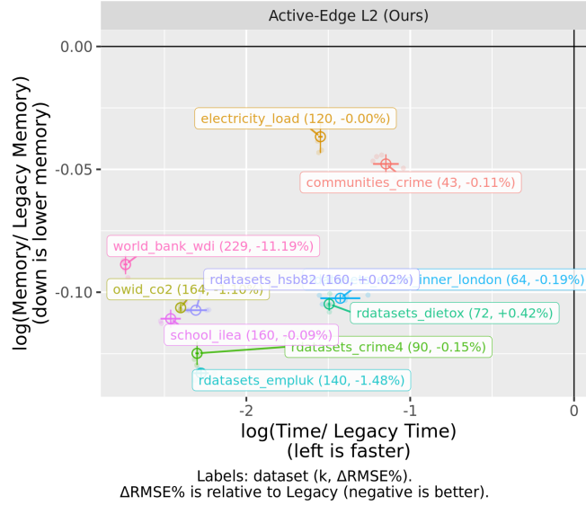
Figure 8: L2 efficiency of active-edge construction relative to the legacy L2 construction.
