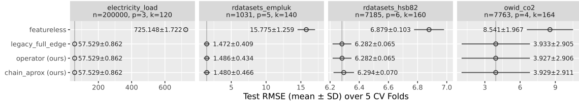
Figure 3: L1 prediction accuracy relative to the legacy L1 solver on the main benchmark panel. The exact operator solver preserves the legacy RMSE, while the chain-specialized approximation trades graph fidelity for speed.
