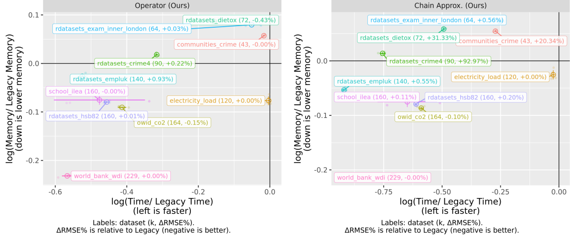
Figure 3: L1 efficiency relative to the legacy solver. Left: exact operator. Right: chain-specialized approximation.
