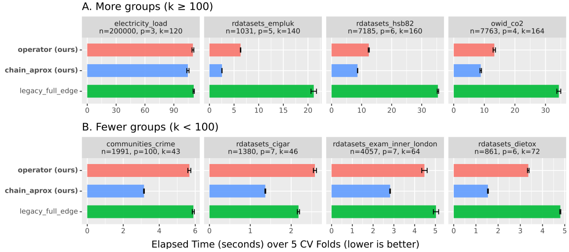
Figure 2: L1 fit time by solver and group-count regime. Active-edge methods reduce the cost of graph fusion when the graph is sparse.
