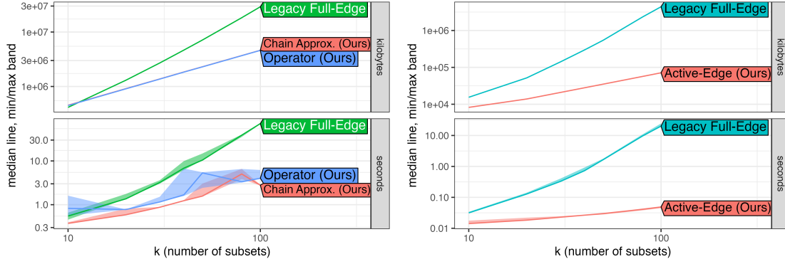
Figure 7: Synthetic scaling experiments for L1 variants (left) and L2 variants (right).
