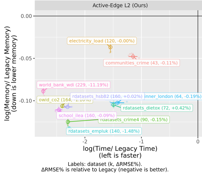
Figure 6: L2 efficiency of active-edge construction relative to the legacy L2 construction.
