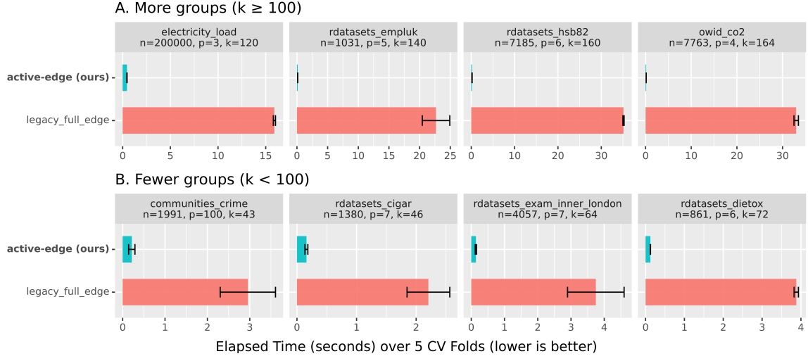
Figure 5: L2 fit time by solver and group-count regime. The active-edge builder reduces augmented-design construction when the graph is sparse.
