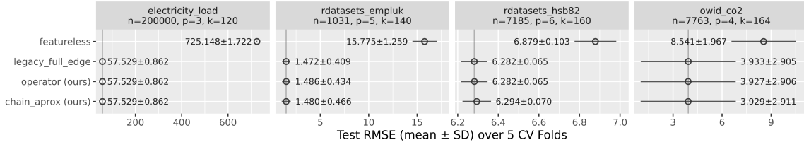
Figure 1: L1 prediction accuracy relative to the legacy L1 solver on the main benchmark panel. The exact operator solver preserves the legacy RMSE, while the chain-specialized approximation trades graph fidelity for speed.
