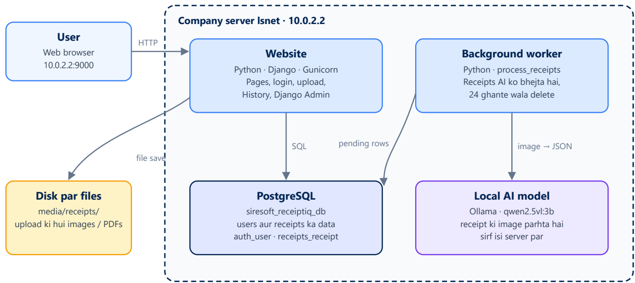
Figure 2 — SireSoft Scan Tool ka architecture
