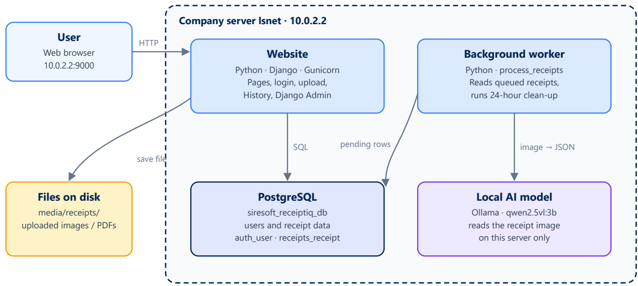
Figure 2 — Architecture of SireSoft Scan Tool
