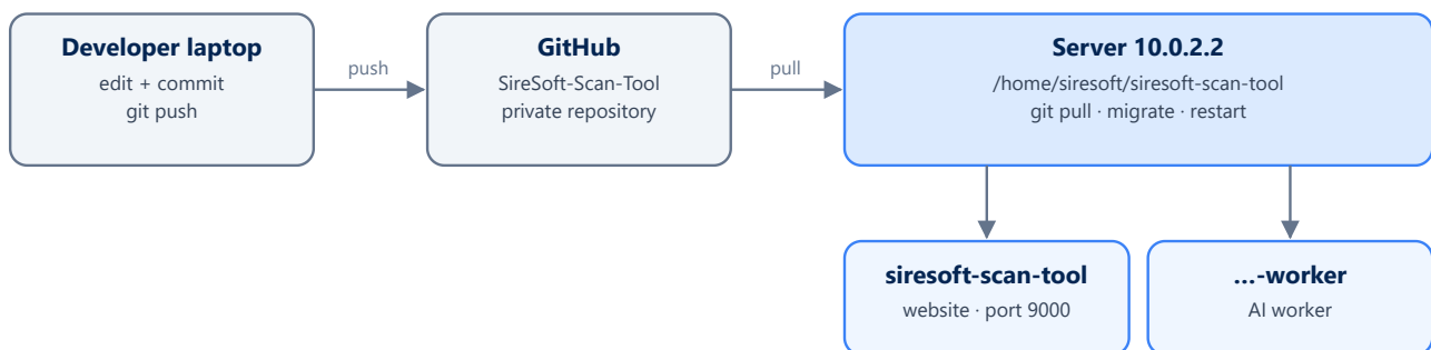
Figure 6 — From code change to running server
