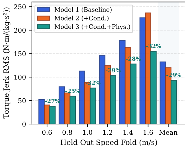
(a) Torque Jerk RMS Across Folds
