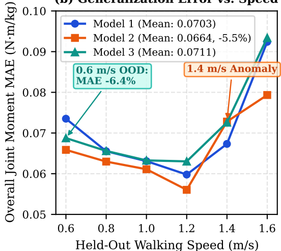
(b) Generalization Error vs. Speed
