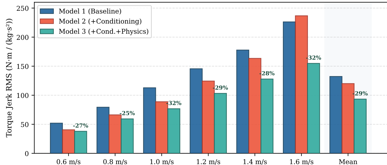
Predicted Torque Jerk Across Leave-One-Speed-Out Folds (Smoothness & Safety Regularization)
