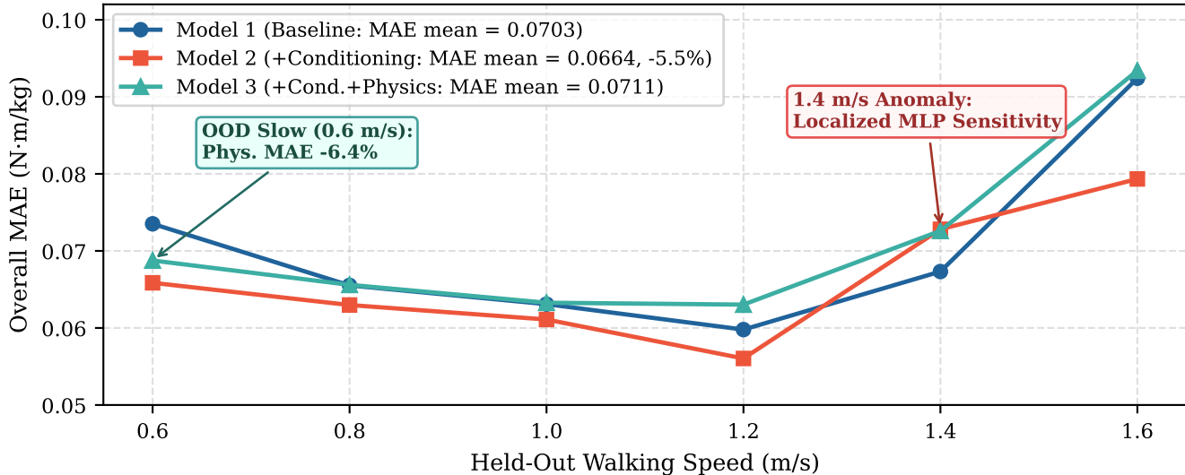
Cross-Speed Generalization: Joint Moment MAE vs. Held-Out Walking Velocity
