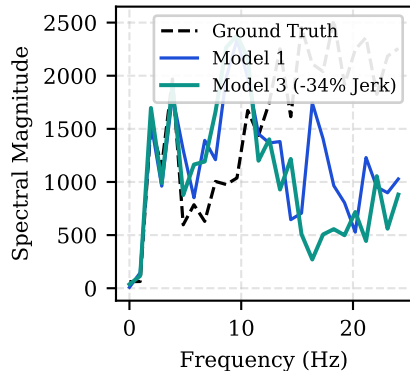
(c) Jerk Spectral Magnitude
