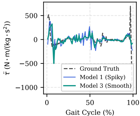
(b) Torque Acceleration ( \ddot{\tau} )
