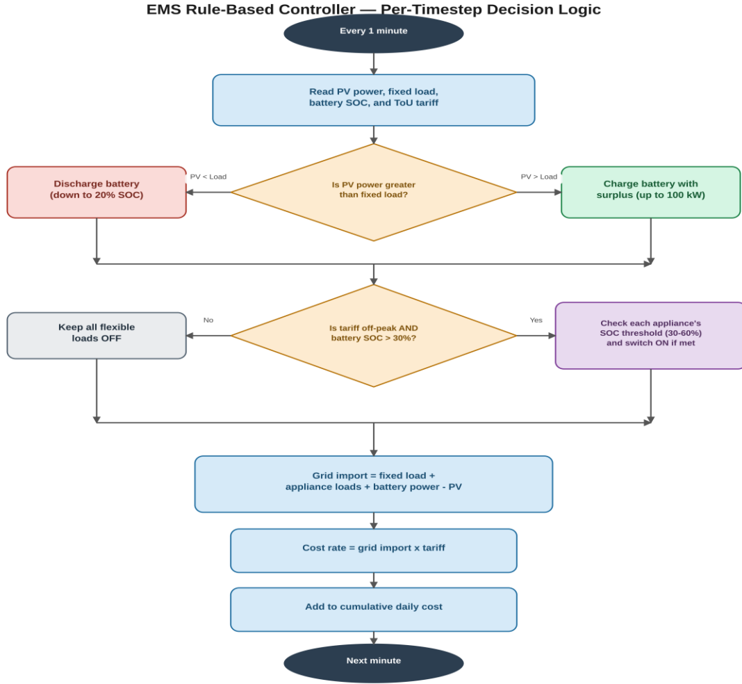
Fig. 17. EMS rule-based controller — per-timestep decision flowchart.
