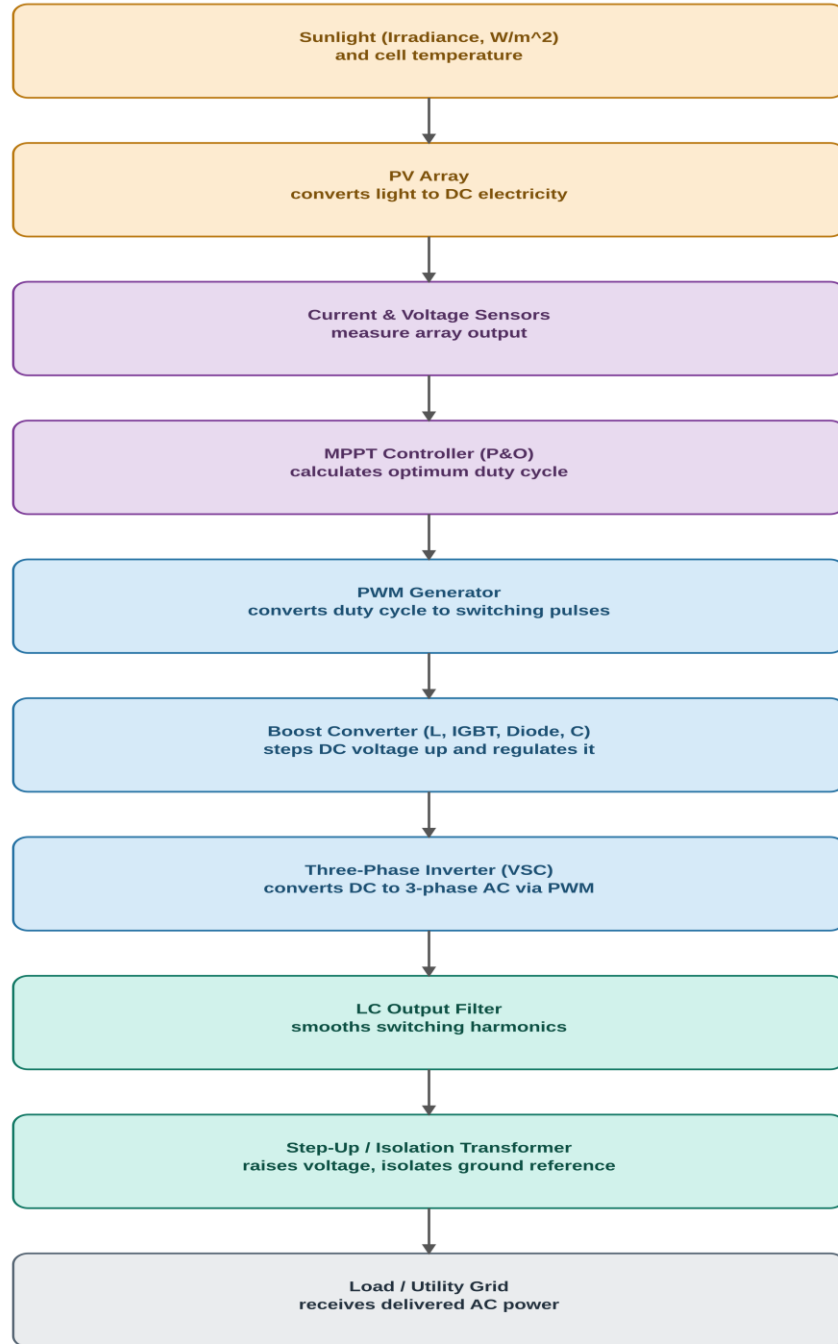
Overall Signal Flow — Sunlight to Grid
