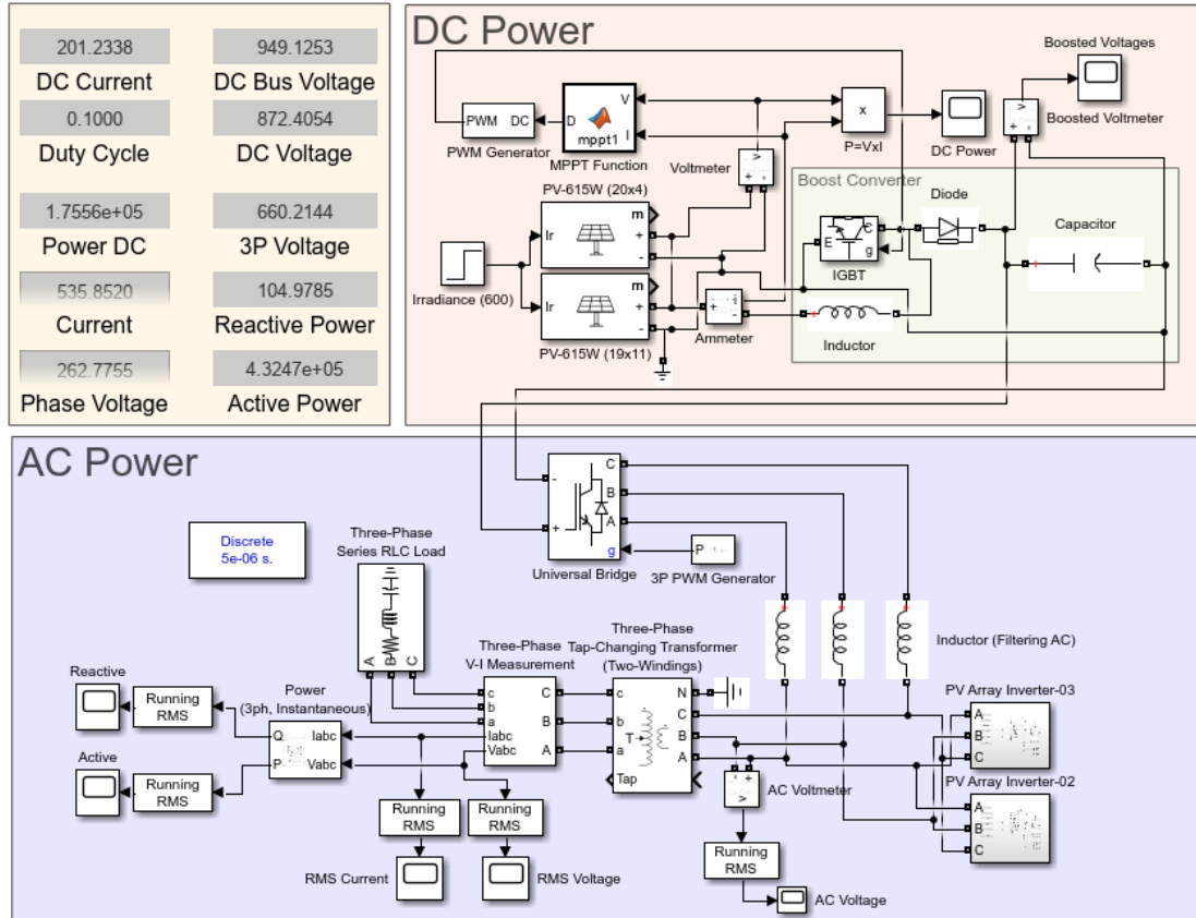
Fig. 3. Complete Simulink implementation of the 520 kW plant (all three chains).
