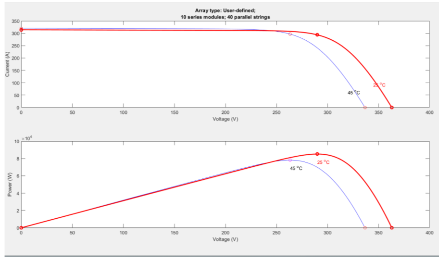
Fig. 4. Simulated I-V and P-V characteristics of the modeled PV array at 25°C and 45°C, 1000 W/m² (direct MATLAB output).
