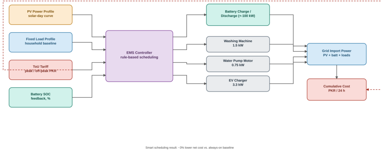
Fig. 16. EMS control-loop architecture — inputs, controller, and outputs.
