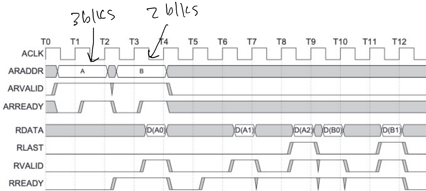
Figure 1-5 Overlapping read bursts
