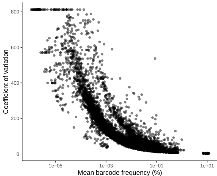
Variability vs abundance across PCR replicates
