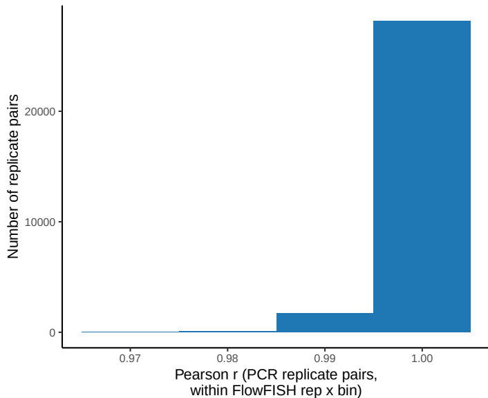
Barcode–frequency correlation between PCR replicates
