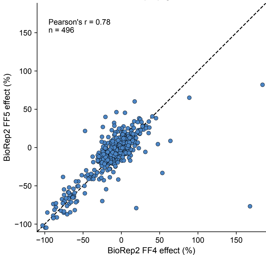
BioRep2 FF4 vs BioRep2 FF5 [axes widened to -110, 188.535] one dot per pegRNA
