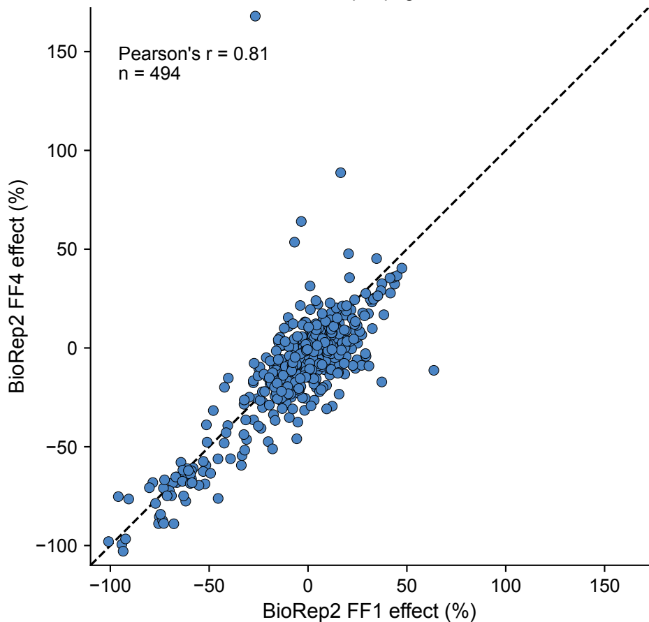
BioRep2 FF1 vs BioRep2 FF4 [axes widened to -110, 172.164] one dot per pegRNA
