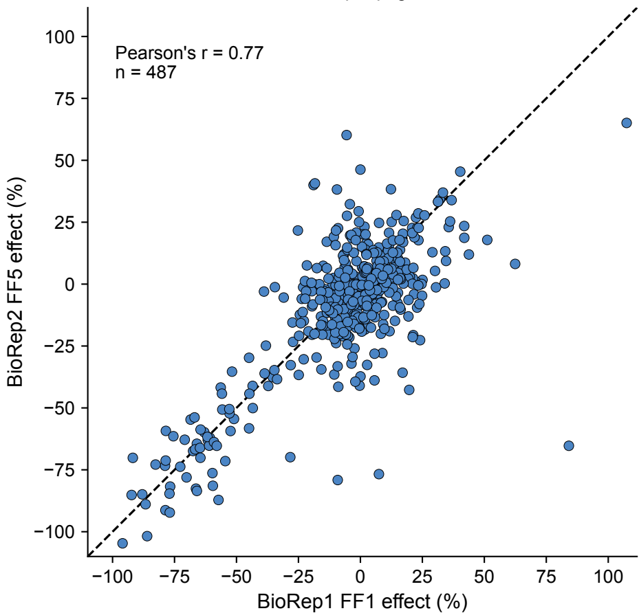
BioRep1 FF1 vs BioRep2 FF5 one dot per pegRNA
