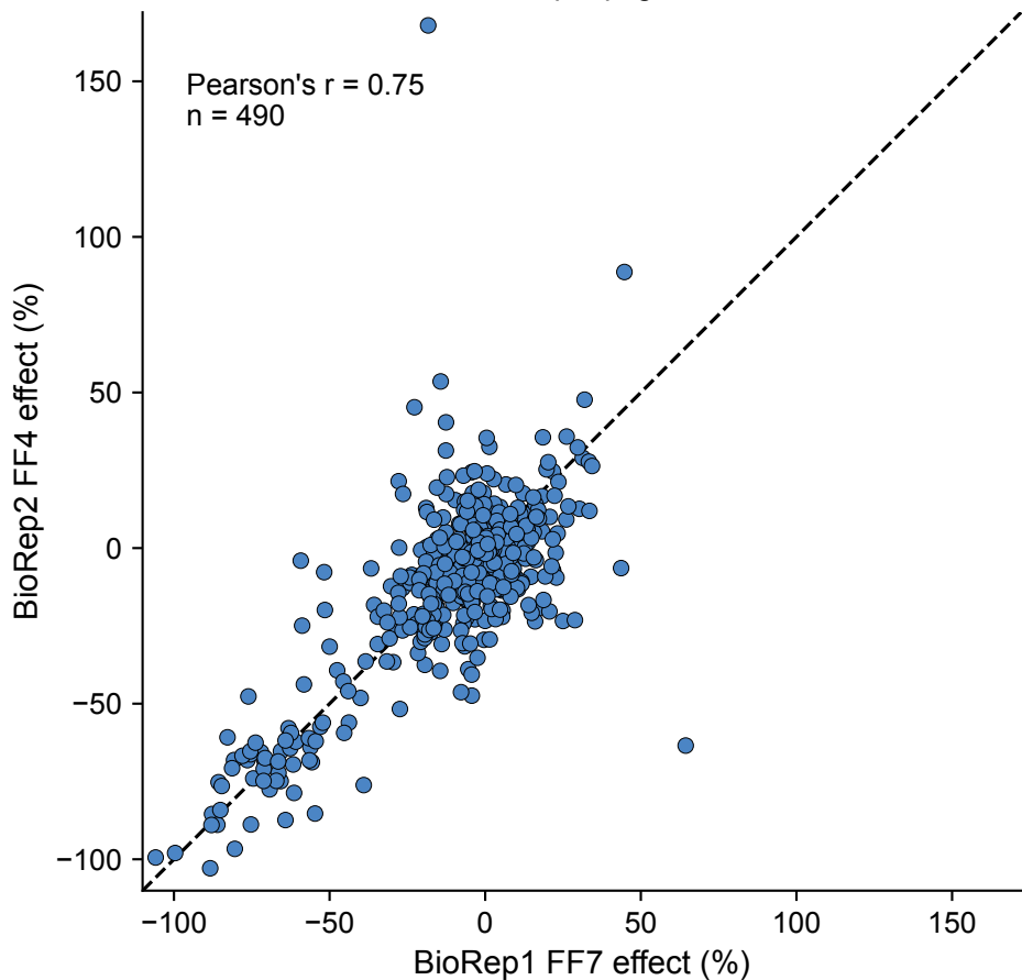
BioRep1 FF7 vs BioRep2 FF4 [axes widened to -110.083, 172.164] one dot per pegRNA
