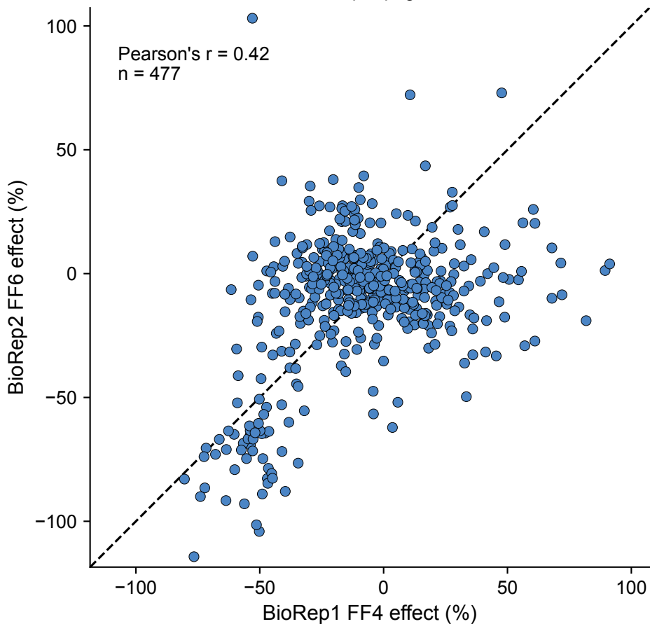
BioRep1 FF4 vs BioRep2 FF6 [excluded: BioRep1 FF4] one dot per pegRNA
