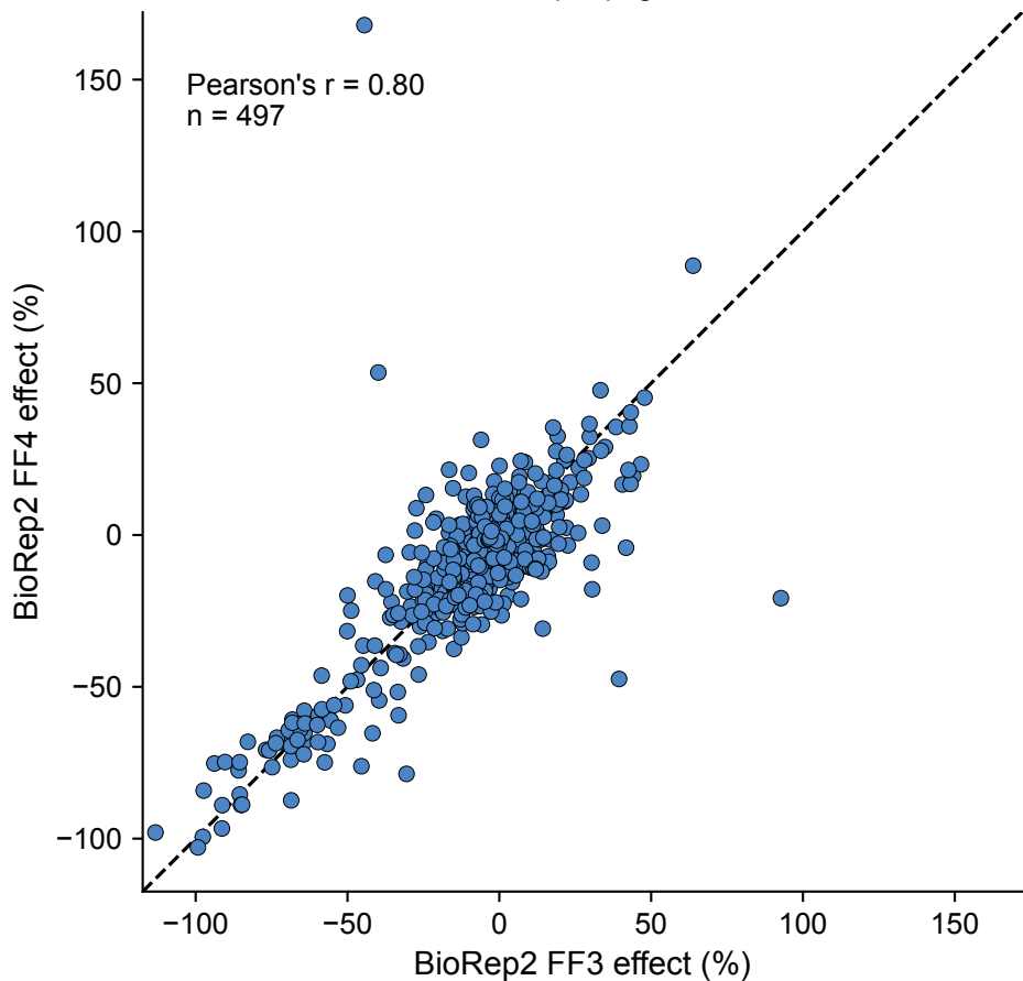
BioRep2 FF3 vs BioRep2 FF4 [axes widened to -117.438, 172.164] one dot per pegRNA
