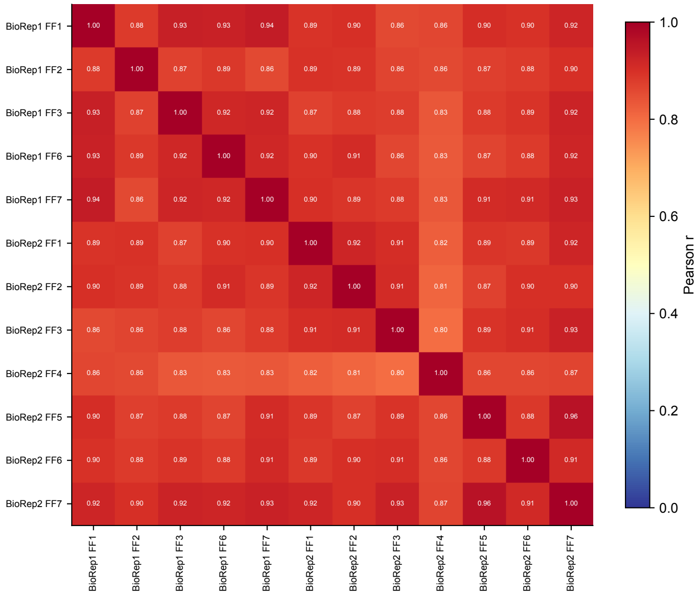
Retained replicates (exclude_replicates applied) Pearson r of per-edit effect between replicates (n=148 edits, mean off-diagonal r=0.89)
