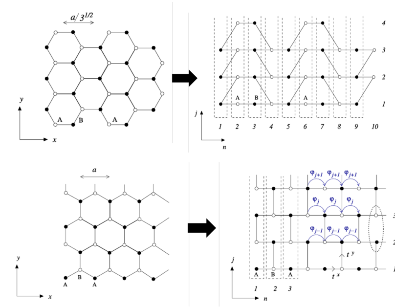
Figure 2: Efficient slicing schemes for different graphene ribbons used to construct an efficient block-tridiagonal Hamiltonian: (a) armchair edge config. and (b) zigzag edge config.
