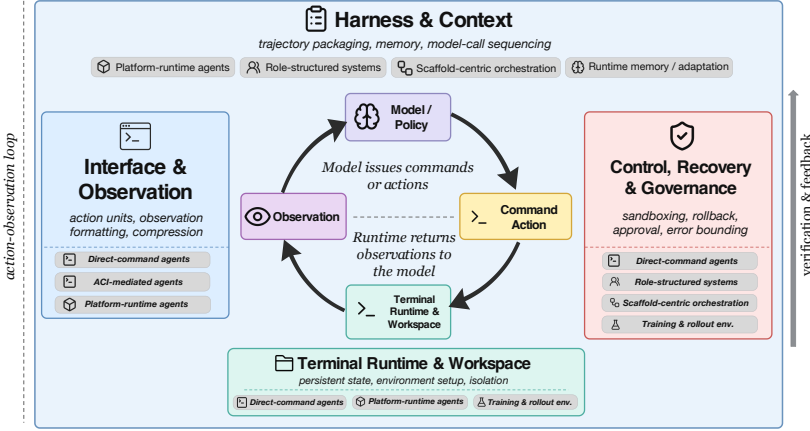
Fig. 5. Layered architecture of terminal-agent systems. The central loop shows action generation, command execution, workspace mutation, and observation return. The surrounding layers show interface shaping, runtime management, control and recovery, and harness-level context management.
