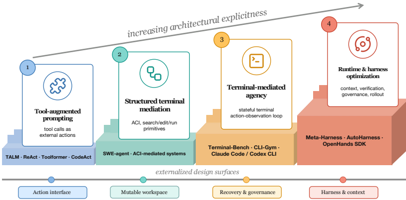
Fig. 4. Technical evolution of terminal-agent architectures. The stages summarize overlapping shifts from tool-augmented prompting to runtime- and harness-centered terminal agency. The bottom axis highlights increasingly explicit design surfaces.
