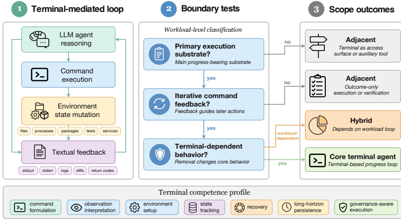
Fig. 3. Operational scope of terminal agents. The figure connects the terminal-mediated action-observation loop, the workload-level boundary tests, the resulting scope categories, and the competence dimensions used throughout the survey.
