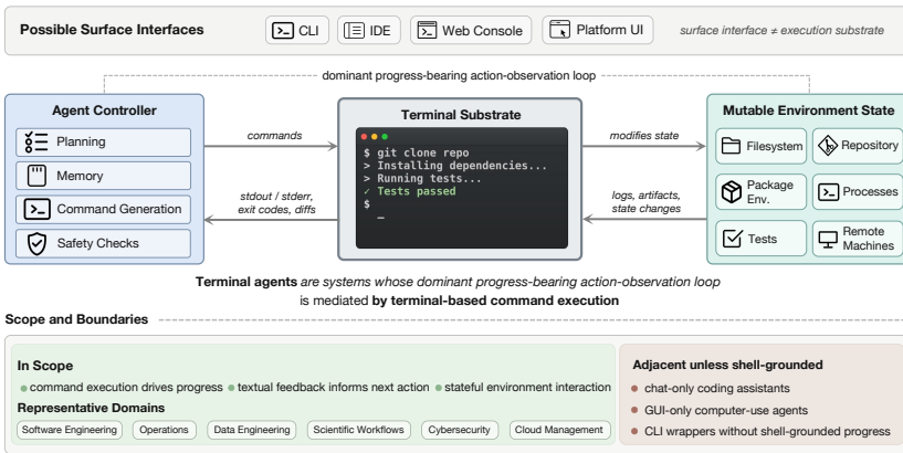
Fig. 1. Definition and scope of terminal agents. Terminal agents are identified by a dominant progress-bearing action-observation loop grounded in terminal-based environments, not by their surface interface. Commands act on mutable environment state, while textual observations such as stdout/stderr, exit codes, diffs, logs, and artifacts provide evidence for subsequent actions.
