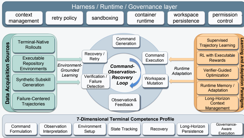
Fig. 6. Terminal competence acquisition ecosystem for terminal agents. Data sources, command-observation-recovery traces, runtime and governance mechanisms, and learning paradigms jointly shape the multi-dimensional terminal competence profile.
