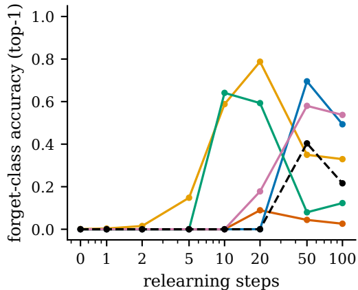
relearning from 5 forgotten images
