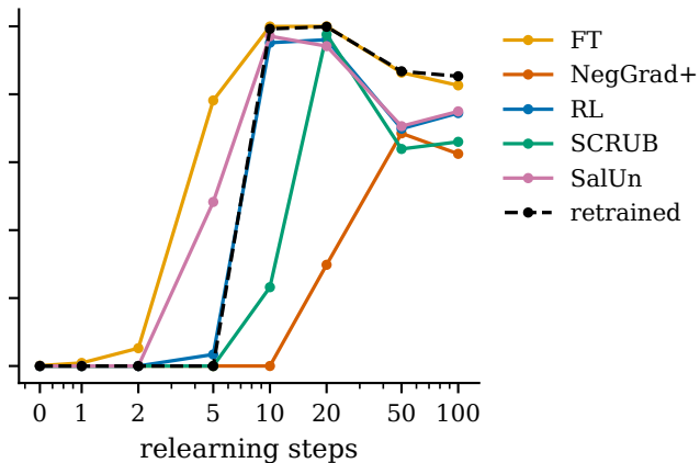
relearning from 100 forgotten images
