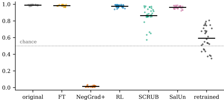
AUROC of the forgotten class's output
