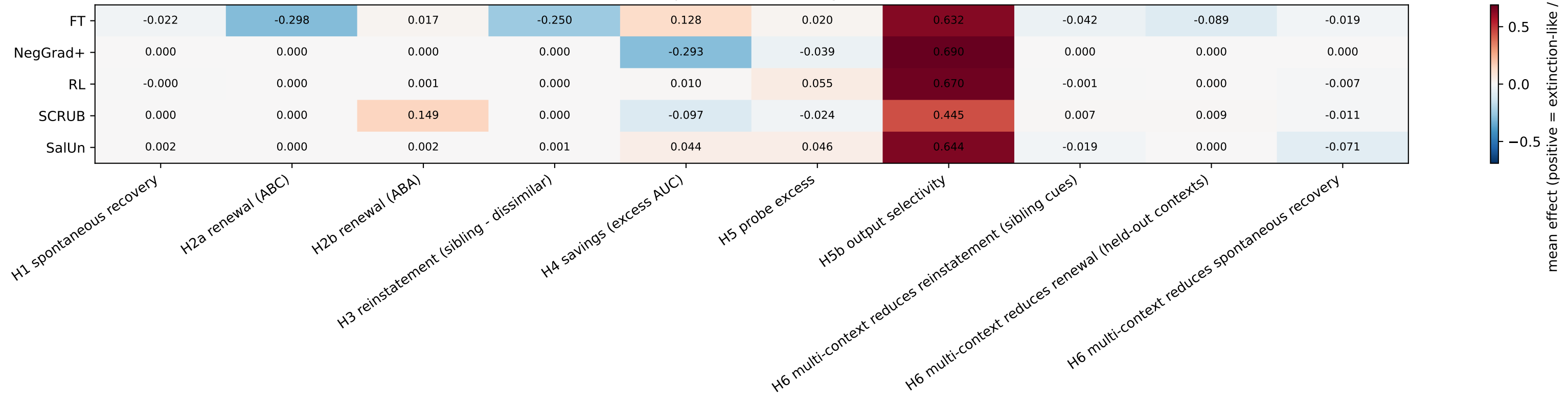
Extinction profile of unlearning methods
