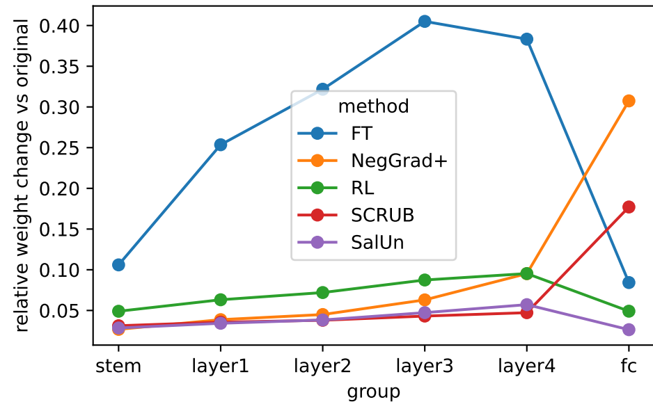
Where unlearning changes the weights
