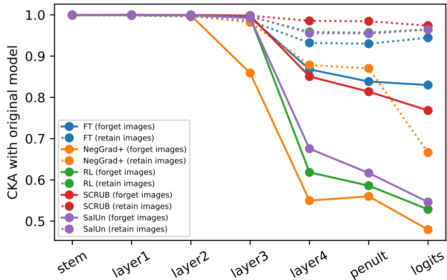
Representation similarity
