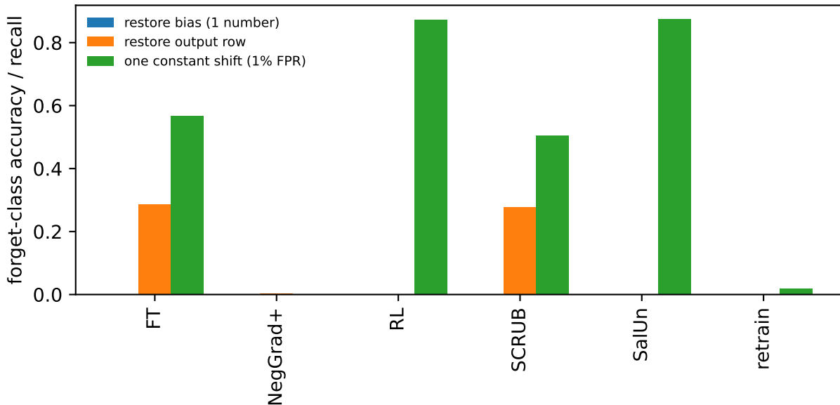
How much of class forgetting sits in the output layer
