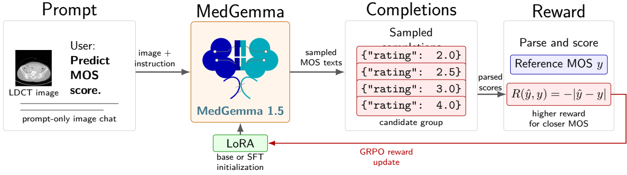
Figure 4.2: GRPO prompt and reward flow for MOS prediction. The model receives the same prompt-only multimodal input but samples a group of candidate MOS responses instead of learning from a fixed assistant target. Parsed scores are compared with the reference MOS using the absolute-error reward, and the reward signal updates the LoRA adapter.
