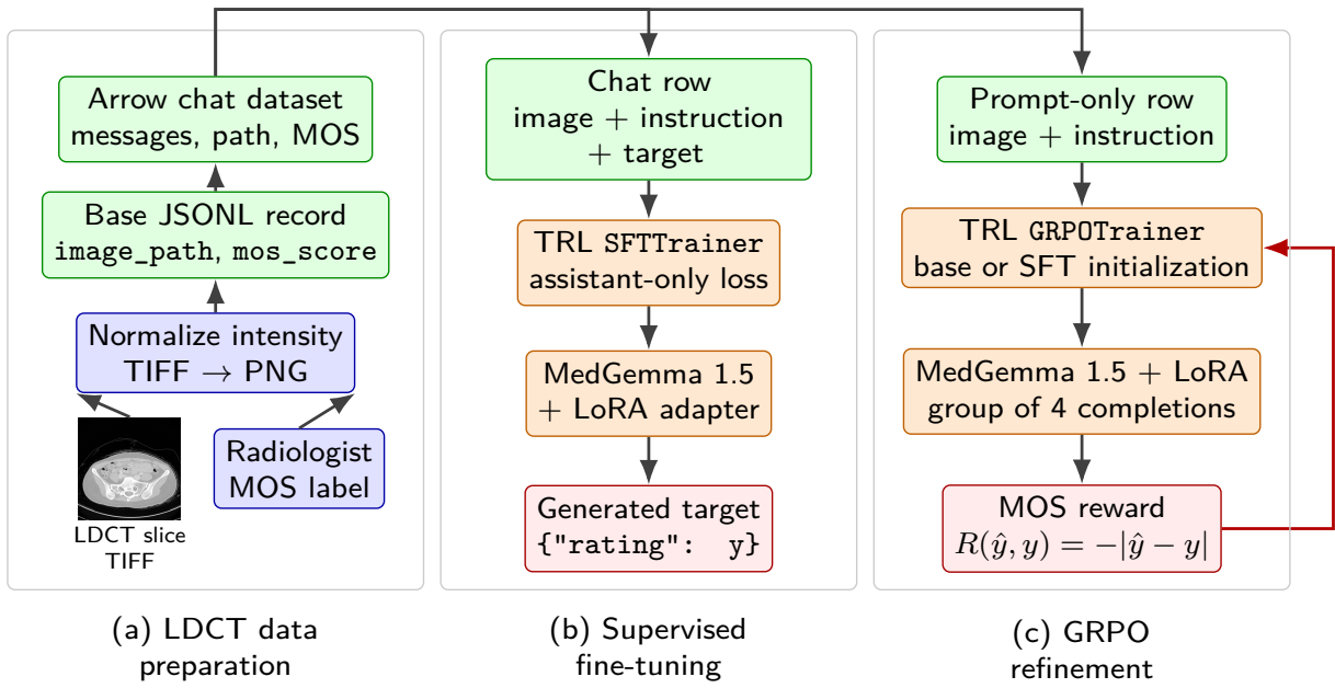
Figure 1.1: Overview of the LDCT MOS prediction pipeline. A shared preprocessing stage converts LDCT images and MOS annotations into normalized PNG paths and JSONL records. Chat-formatted Arrow datasets support the SFT and GRPO paths used for generative adaptation.
