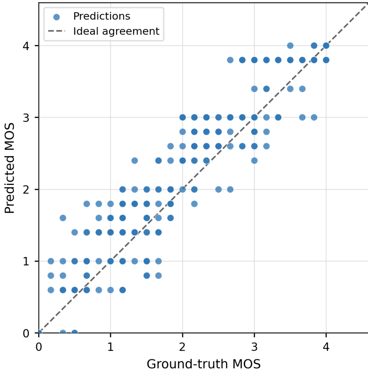
Figure 6.1: Predicted versus ground-truth MOS for the selected SFT run. The dashed line denotes ideal agreement. Overall, 71.3% of predictions fall within \pm 0.5 MOS of the reference score.
