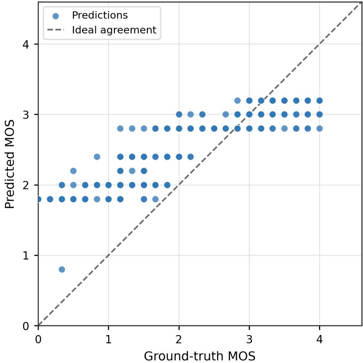
Figure 6.2: Predicted versus ground-truth MOS for the selected SFT-initialized GRPO run. The discrete prediction bands indicate remaining score-range compression after reward-based refinement. Overall, 43.3% of predictions fall within \pm 0.5 MOS of the reference score.
