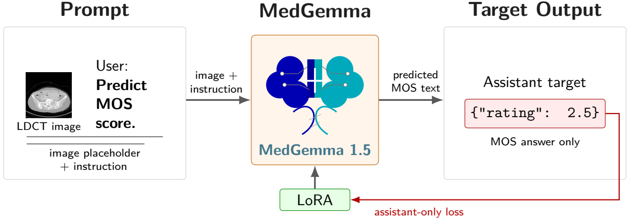
Figure 4.1: SFT prompt construction for MOS prediction. Each LDCT image is paired with a user instruction and the assistant target contains only the MOS value in a compact JSON format. During fine-tuning, the loss is applied to the assistant response while LoRA adapts the MedGemma VLM.
