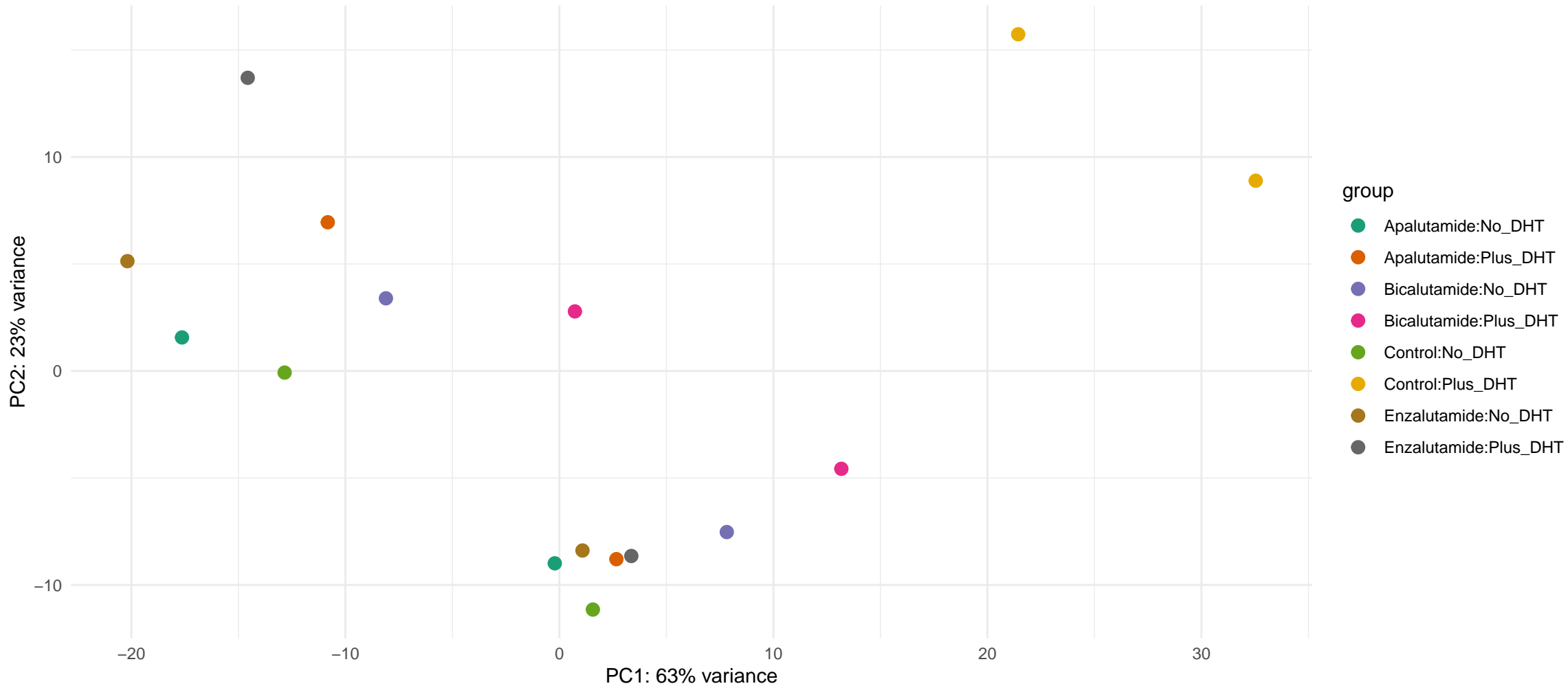
PCA of Samples (VST-transformed counts)
