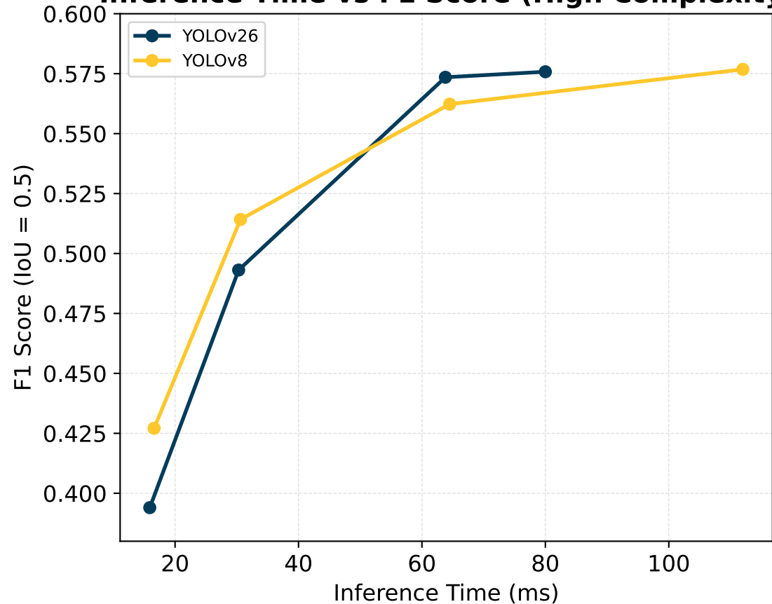
Inference Time vs F1 Score (High Complexity)
