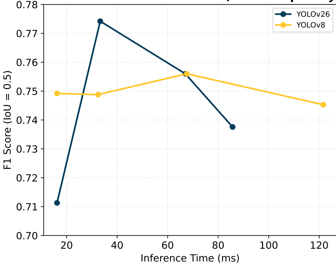
Inference Time vs F1 Score (Low Complexity)
