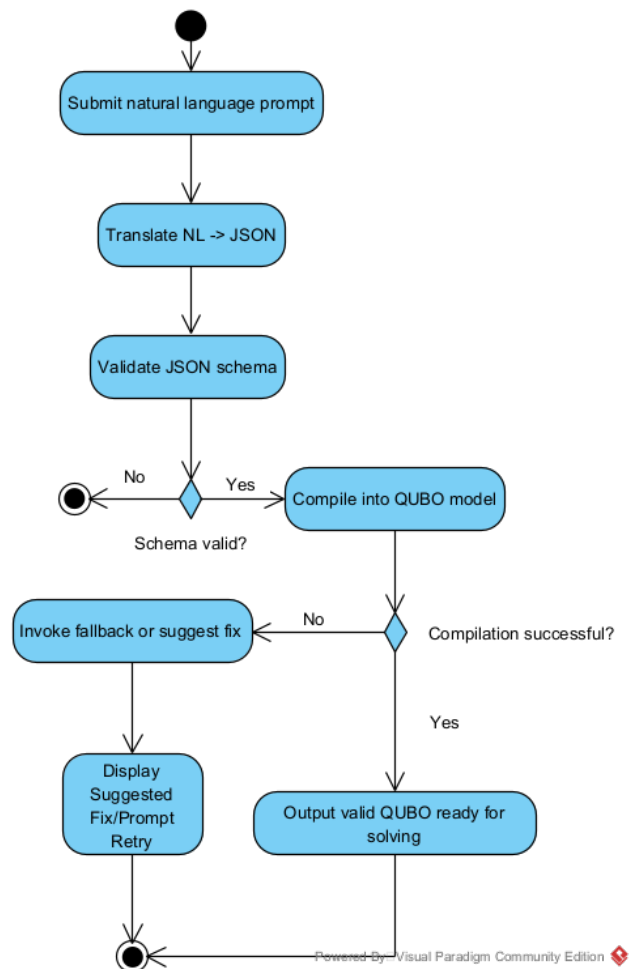
Figure 6.2: Activity Diagram for ucTranslatePrompt ( UC_1 )
