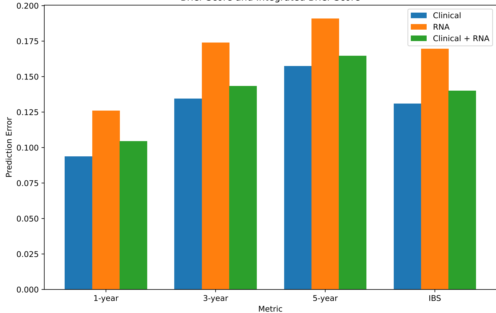
Brier Score and Integrated Brier Score
