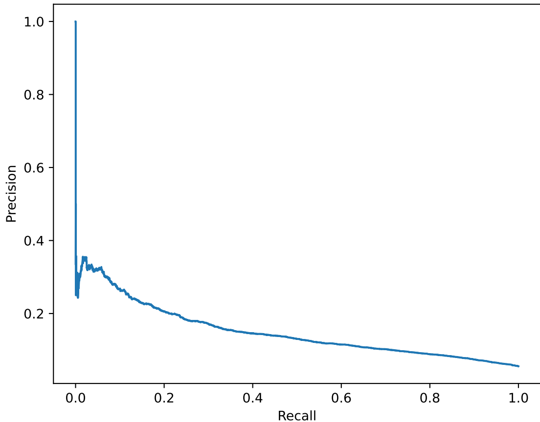
EXP-0 [abstracted] holdout PR curve (PR-AUC=0.1500)
