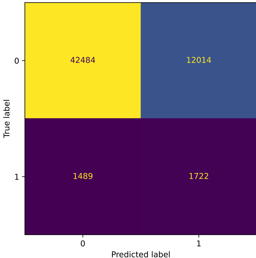
EXP-0 [normalized] holdout confusion matrix (threshold=0)
