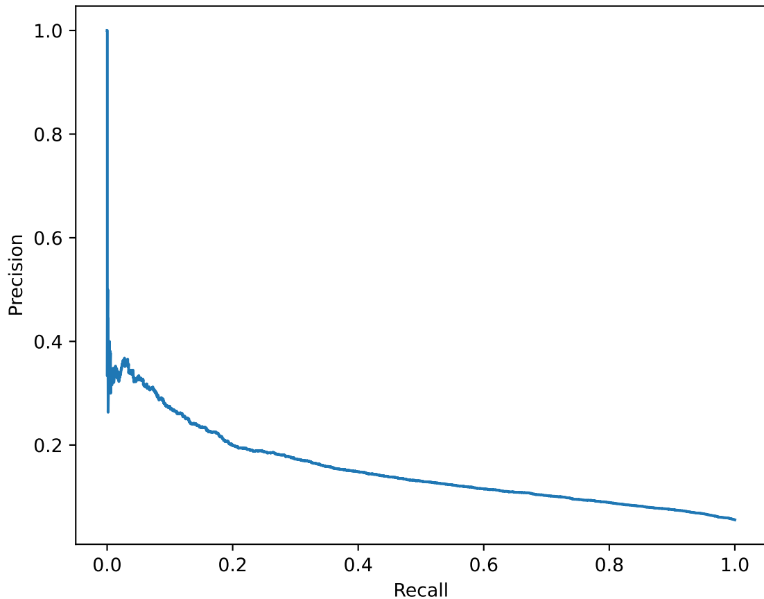
EXP-0 [normalized] holdout PR curve (PR-AUC=0.1524)
