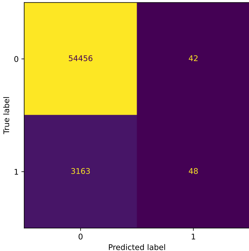
EXP-1 [abstracted] holdout confusion matrix (threshold=0
