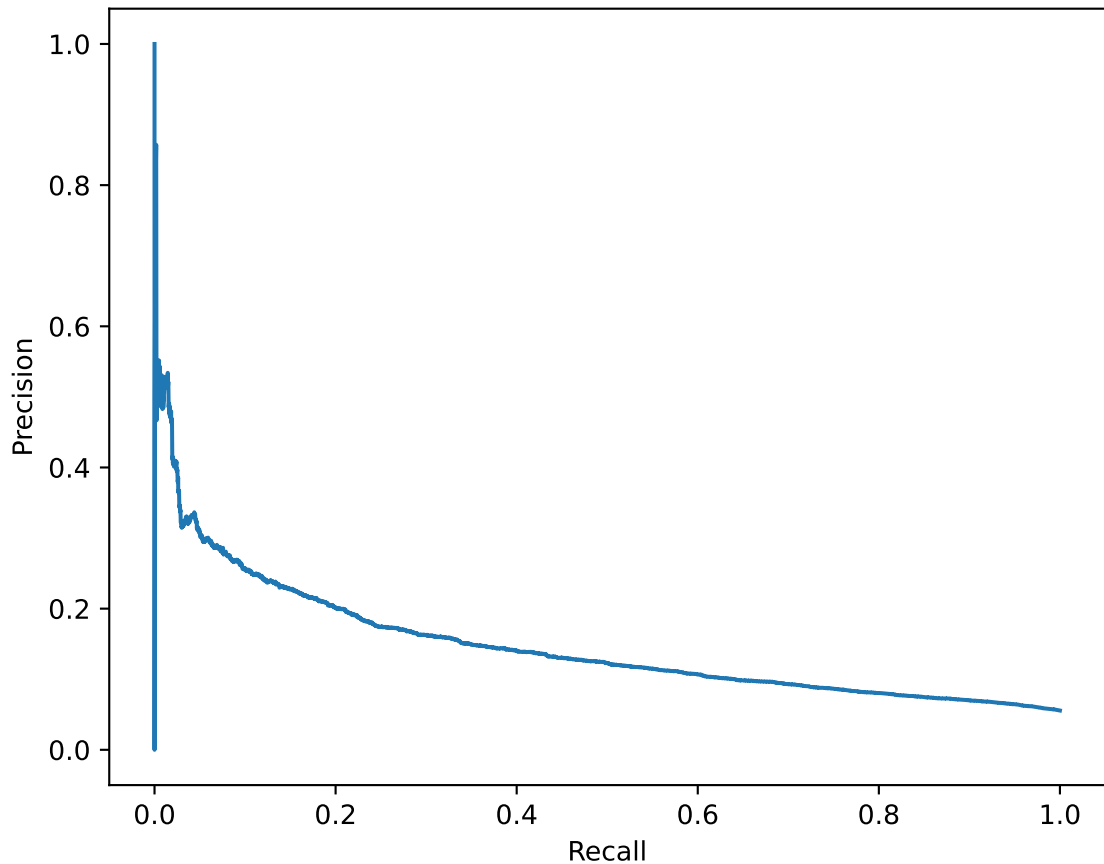
EXP-1 [abstracted] holdout PR curve (PR-AUC=0.1477)
