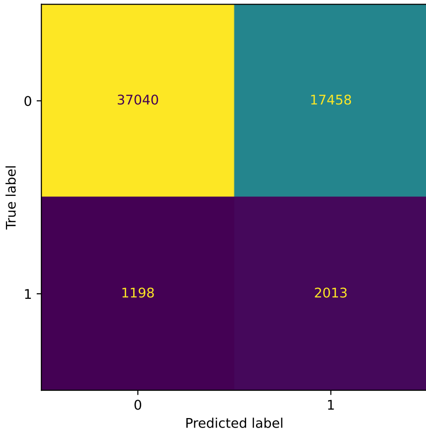
EXP-2 [abstracted] holdout confusion matrix (threshold=0
