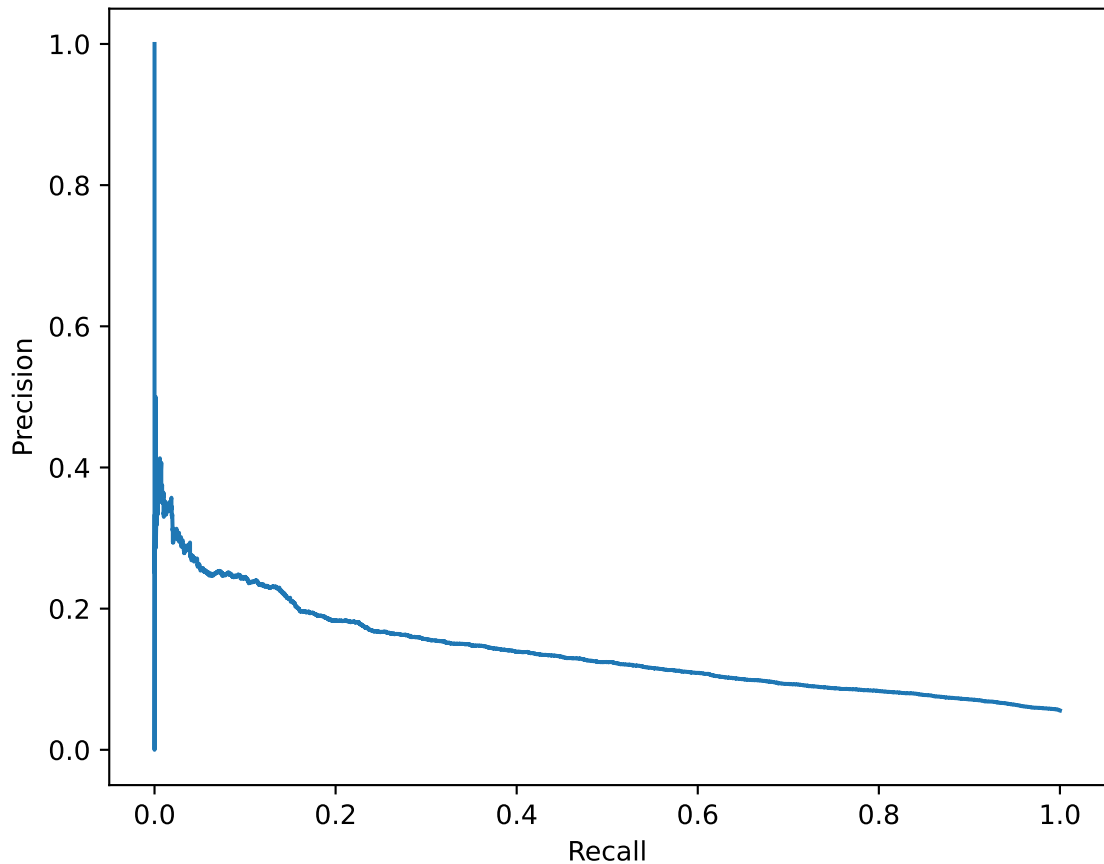
EXP-2 [abstracted] holdout PR curve (PR-AUC=0.1391)
