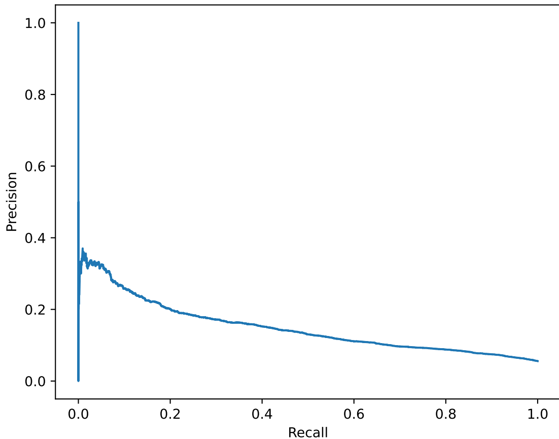
EXP-2 [normalized] holdout PR curve (PR-AUC=0.1492)
