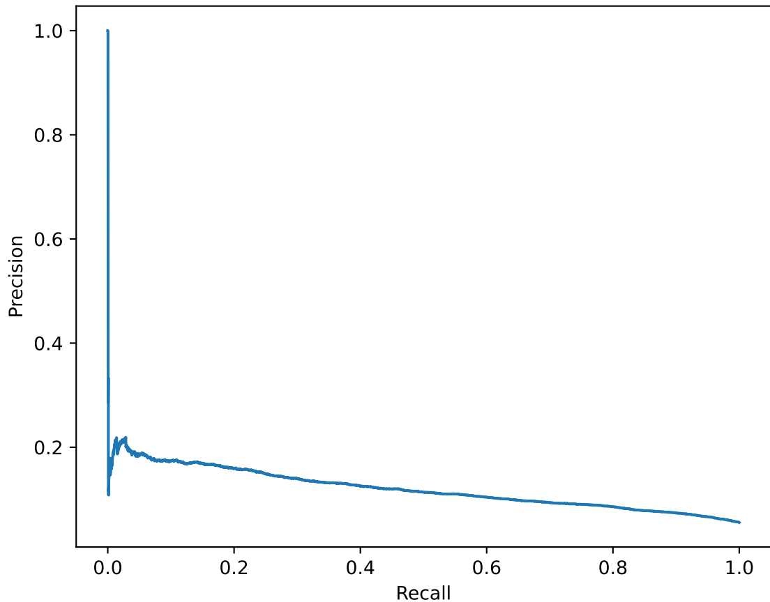
EXP-6 [normalized] holdout PR curve (PR-AUC=0.1204)
